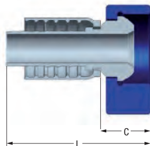
Male Hammer Union Fig. 1502 integral fitting with Lug Nut ( One Piece No-Skive ) use with Alfabiotech 4000, 5000 and Flexor Rig Hoses
