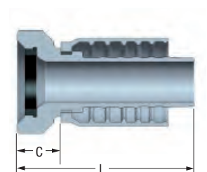
Female Hammer Union Fig. 1502 integral fitting with Rubber Ring ( One Piece No-Skive ) use with Alfabiotech 4000, 5000 and Flexor Rig Hoses
